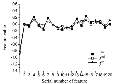
Fig. 8. Feature value (rubbing left, CH1).
